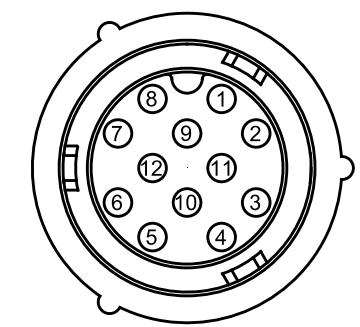
CONTACT END VIEW 12 PIN FEMALE
