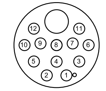
CONTACT END VIEW 12 PIN MALE
